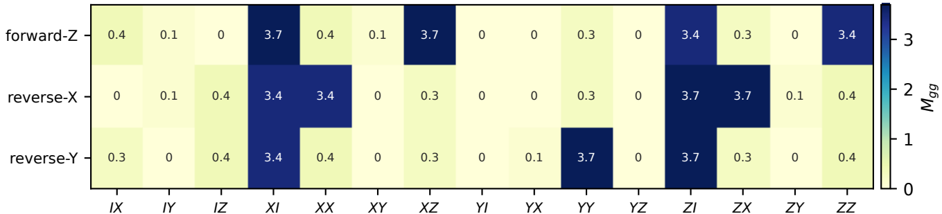
diagonal coherent sensitivity, all 15 generators (invariant labels, F_0 = 0.9 )
