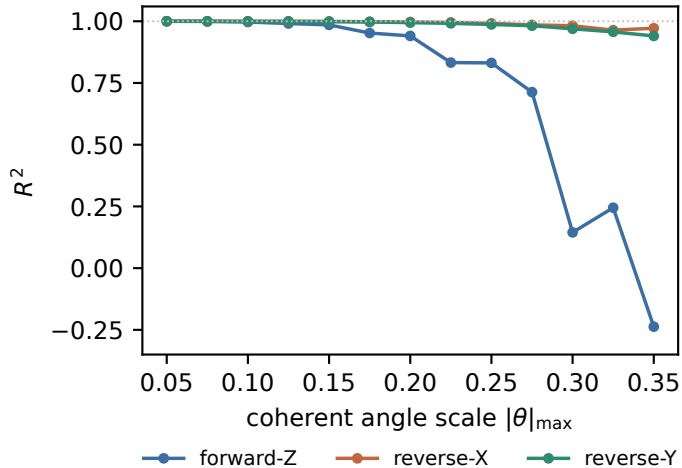
(b) regime of validity
