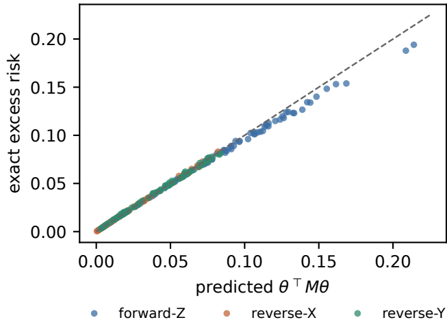
(a) closed form predicts excess risk
