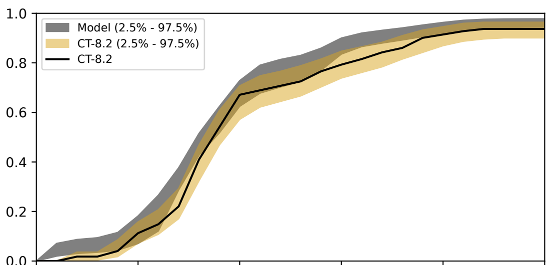
Age (Ma)
