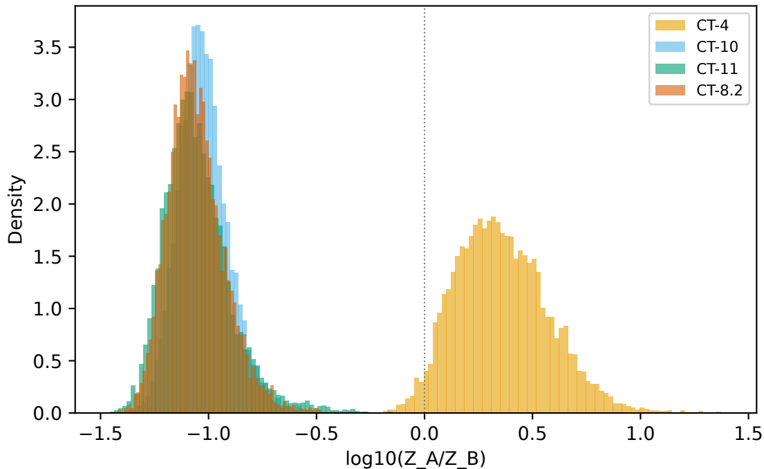
CT-2 alternative parents — zircon fertility (log10, vmax)
