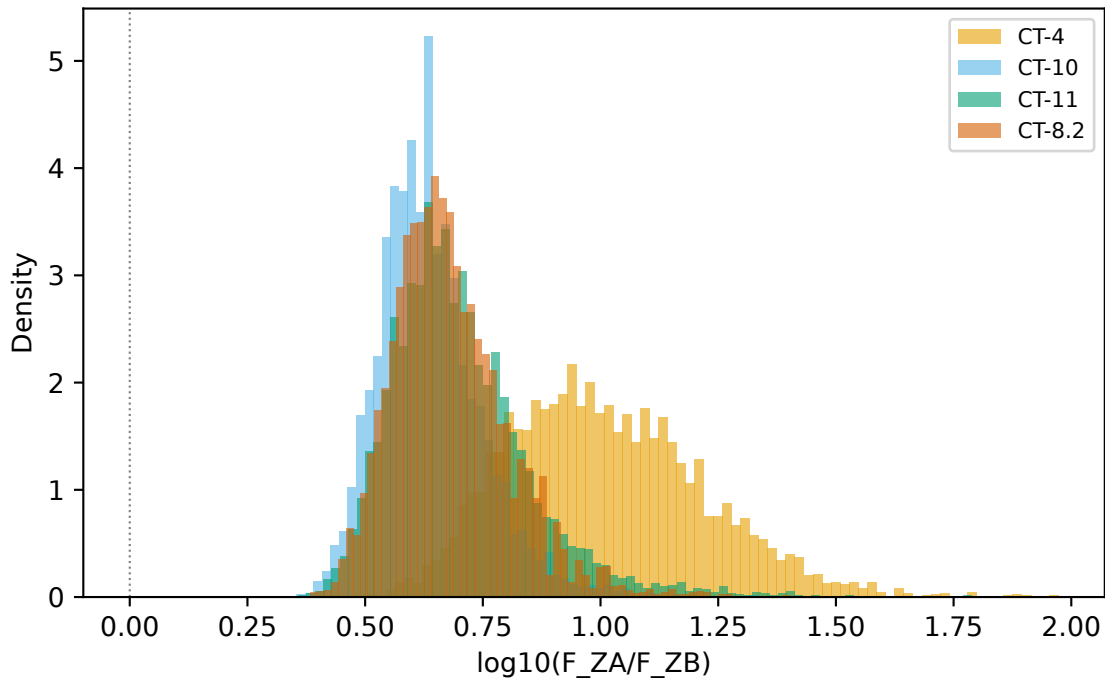
CT-2 alternative parents — zircon flux (log10, vmax)
