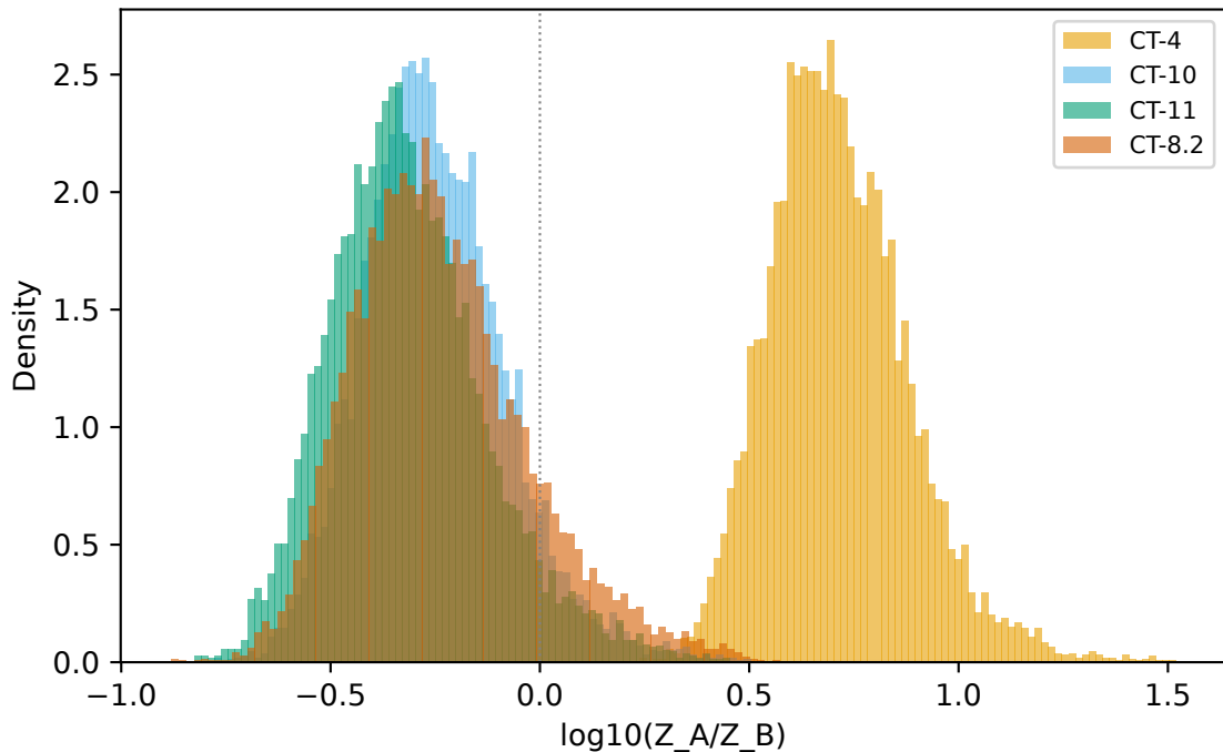
CT-9 alternative parents — zircon fertility (log10, r2kde)
