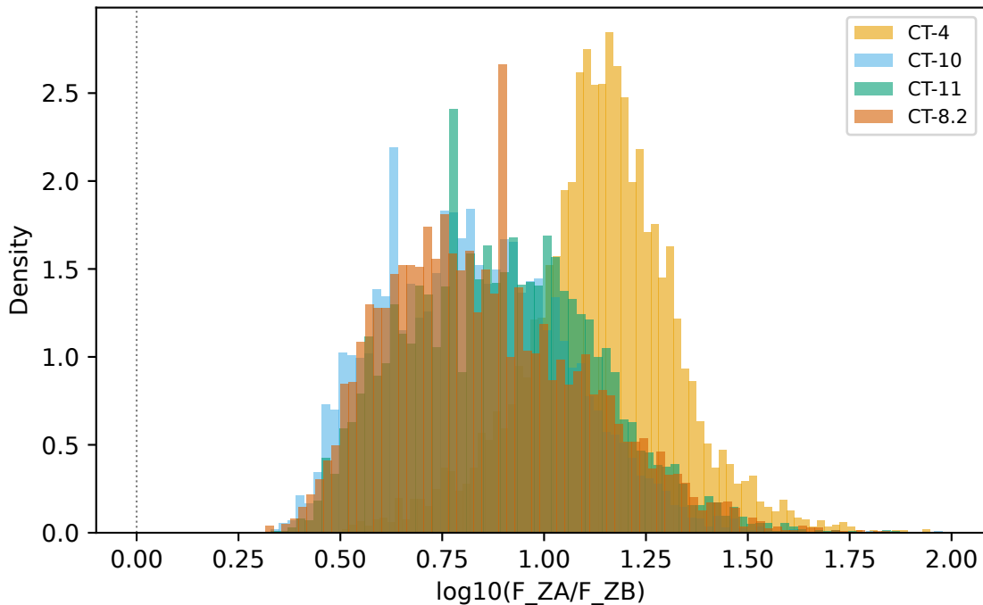
CT-9 alternative parents — zircon flux (log10, vmax)
