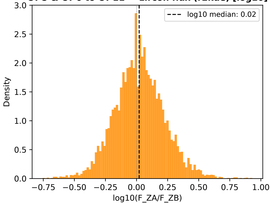
CT-5 & CT-6 to CT-11 — zircon flux (r2kde) [log10]
