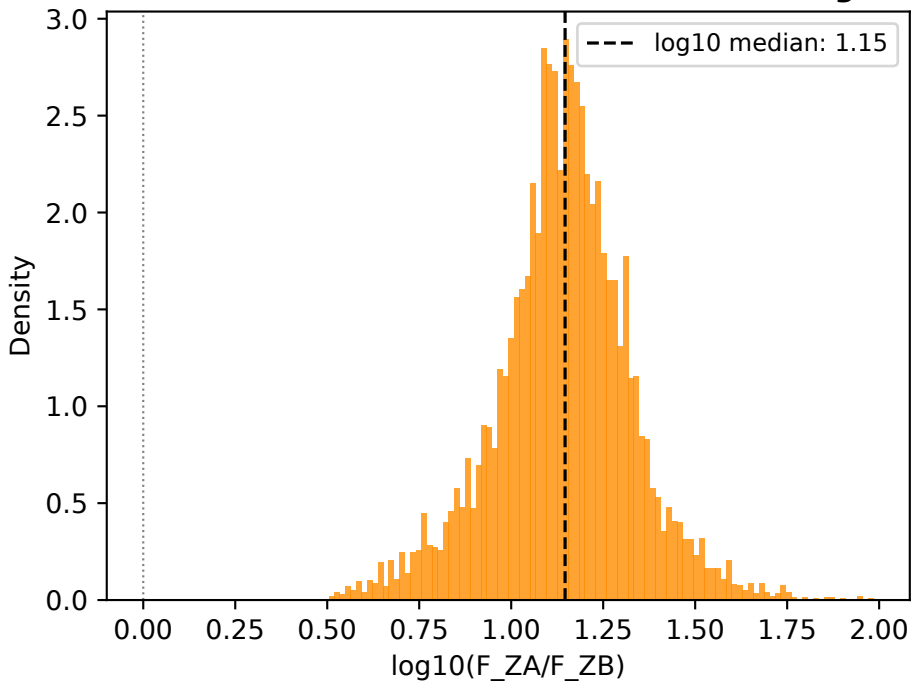
CT-4 & CT-3* to CT-9 — zircon flux (vmax) [log10]
