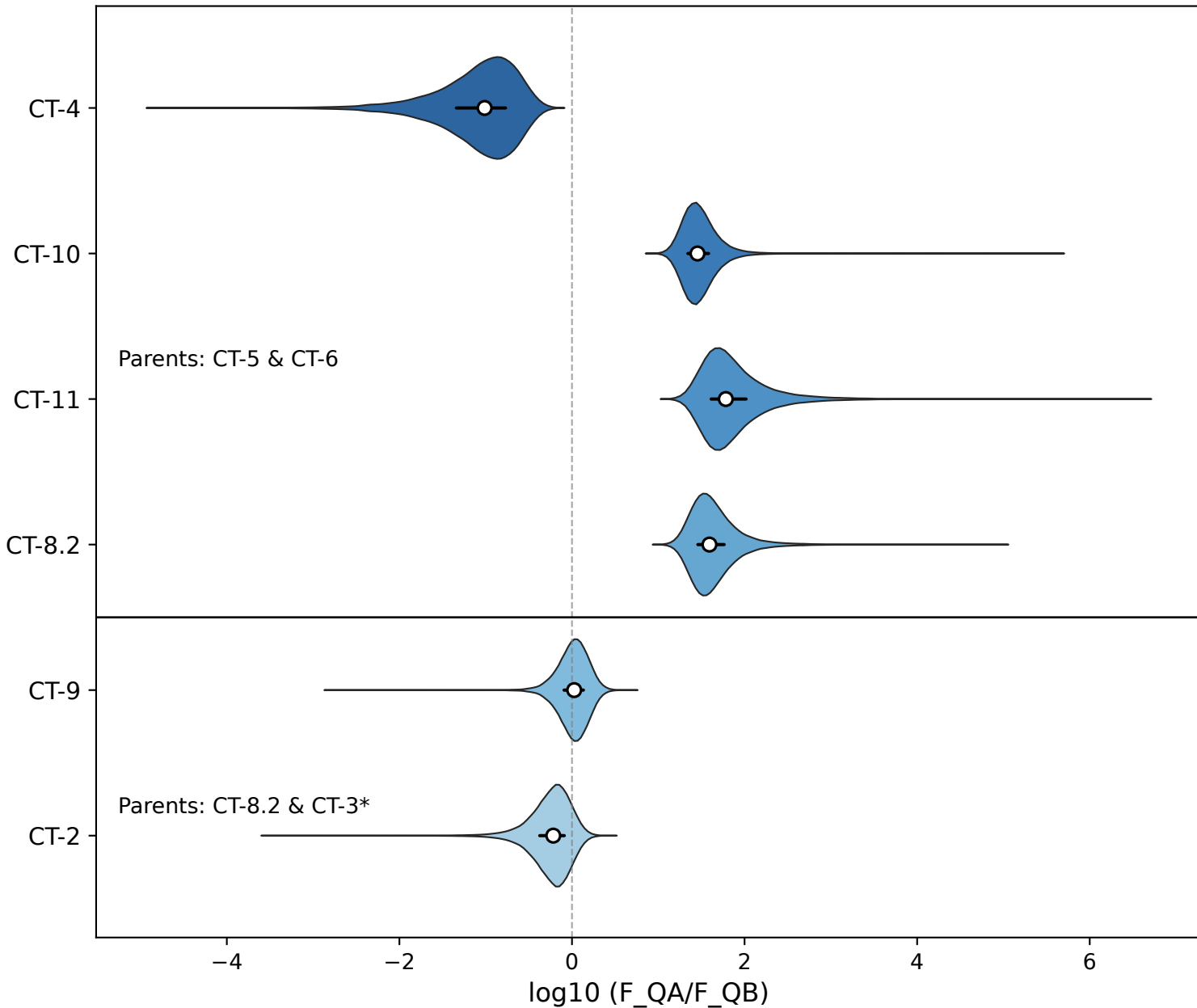
Quartz flux by child sample (log10)
