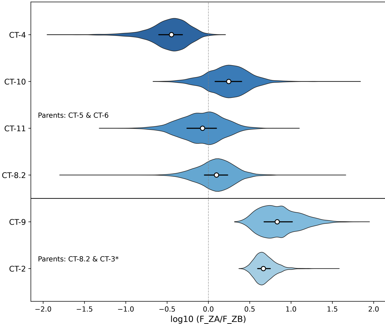
Zircon flux by child sample (log10) — vmax
