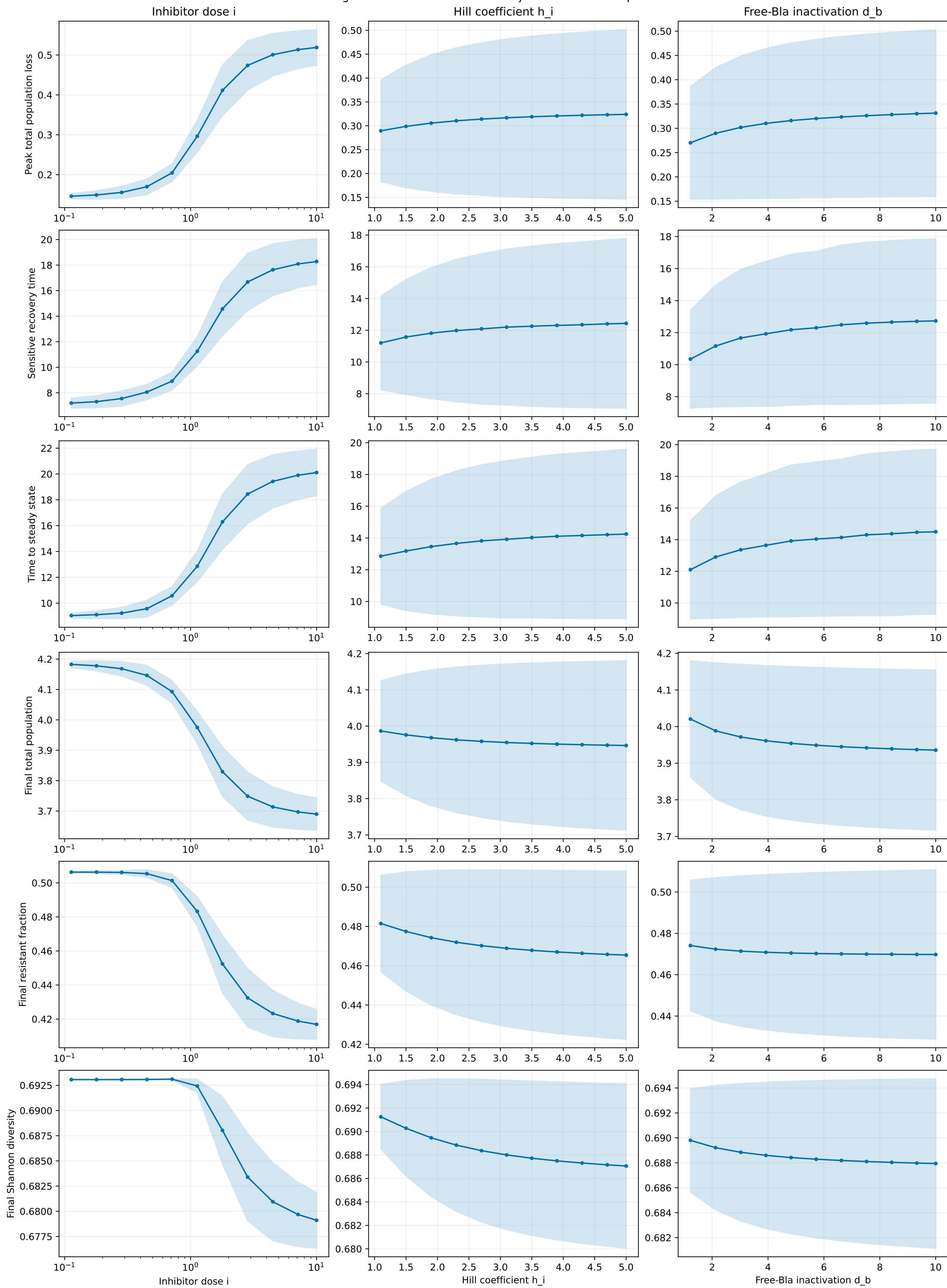
Marginal binned effects across the joint inhibitor sweep
