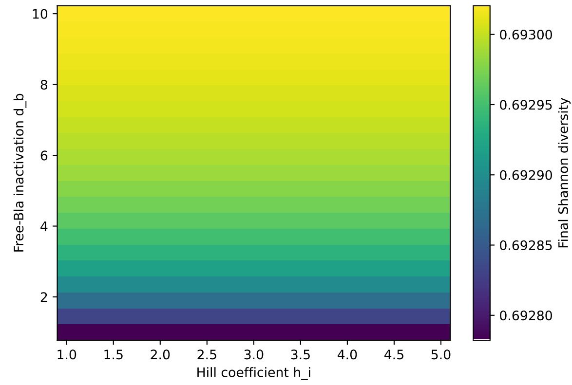
Hill coefficient h_i \times Free-Bla inactivation d_b Fixed: Inhibitor dose i=1
