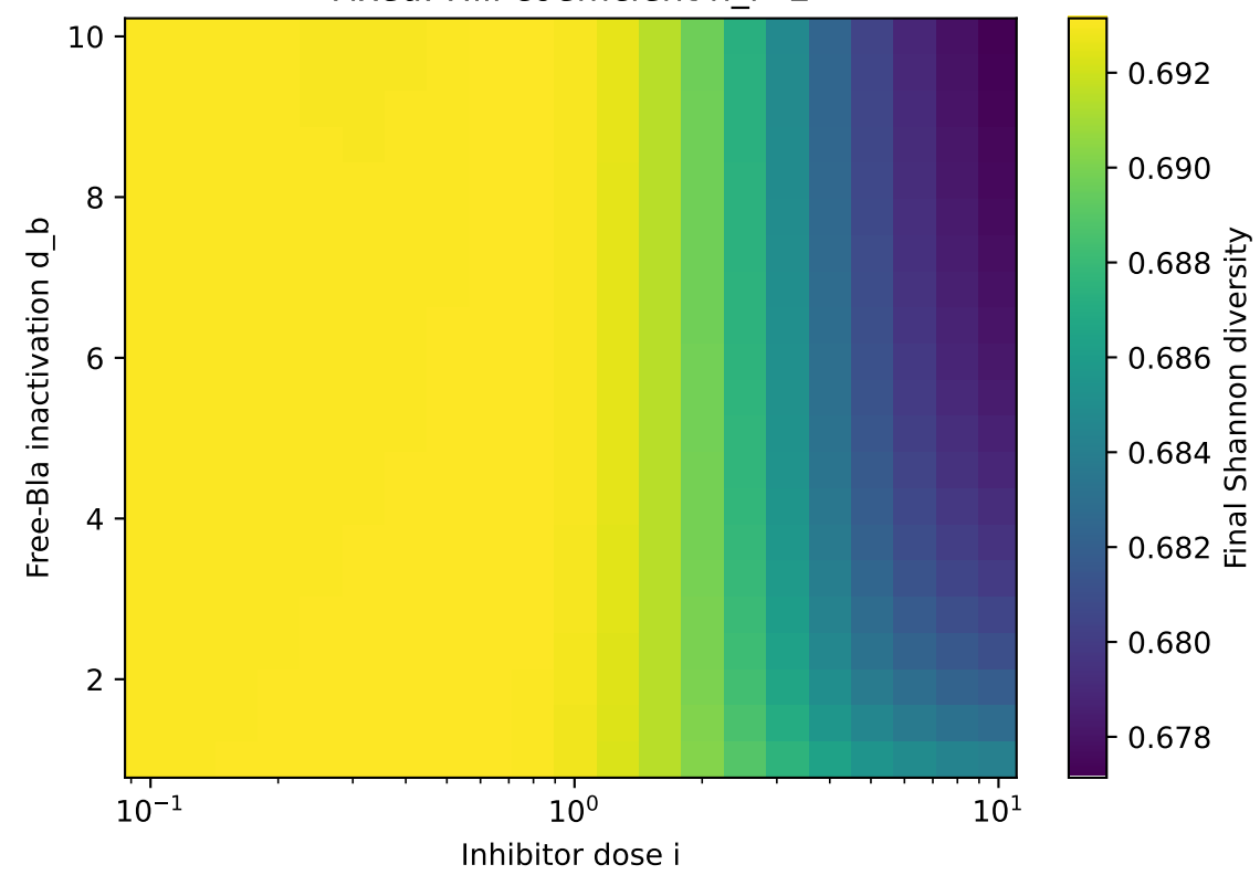
Inhibitor dose i \times Free-Bla inactivation d_b Fixed: Hill coefficient h_i=2
