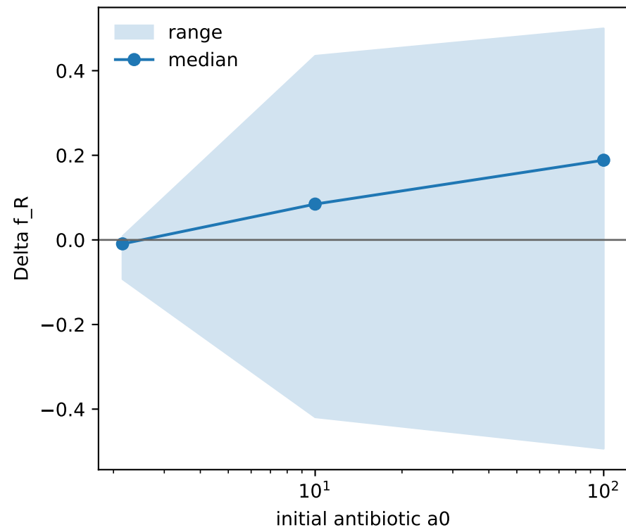
Selection effect across atlas
