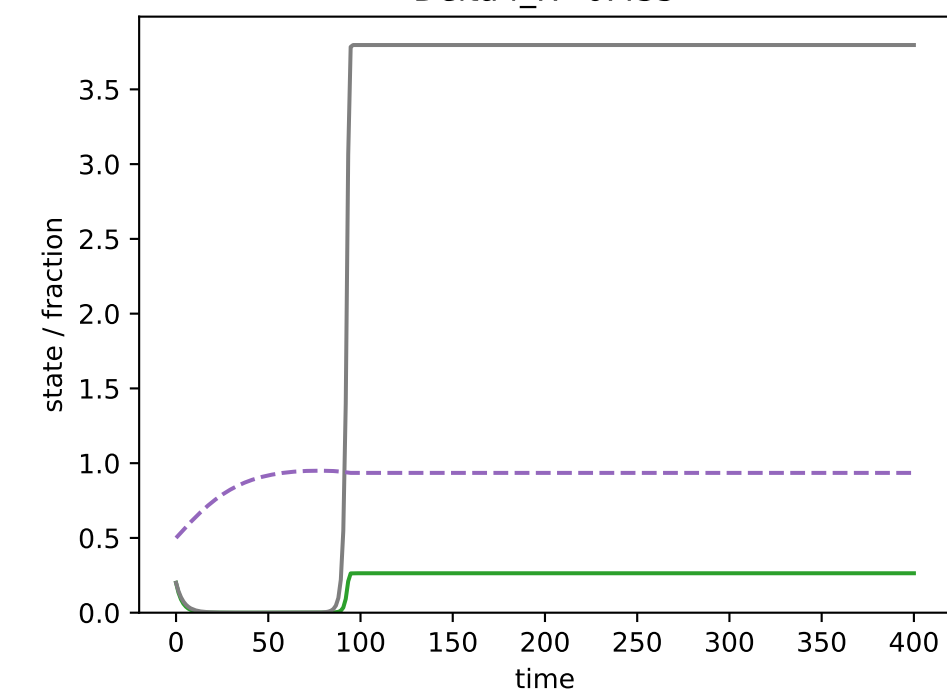
a0=100: most resistant enriched i=0.316, h_i=2, d_b=10 Delta f_R=0.500
