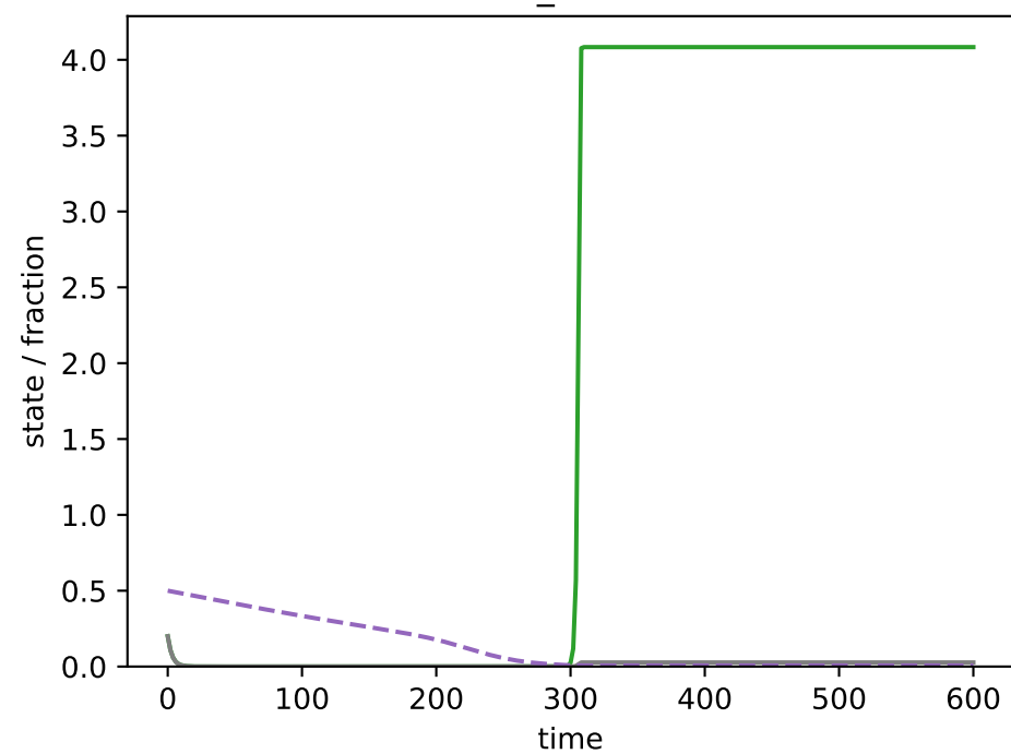
a0=100: most susceptible enriched i=10, h_i=5, d_b=10 Delta f_R=-0.493
