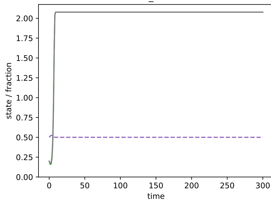
a0=10: near neutral i=1.26, h_i=3.7, d_b=1 Delta f_R=-0.007
