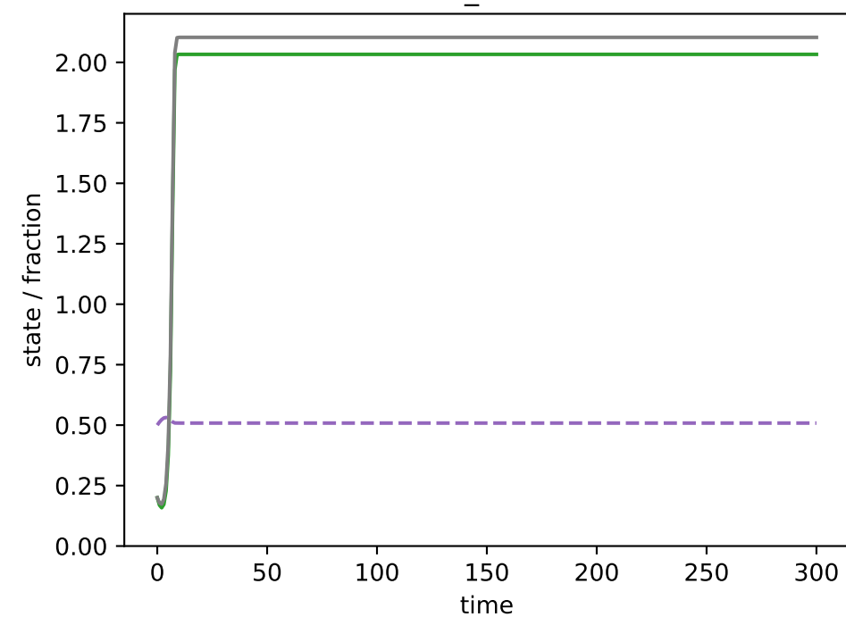
a0=10: most resistant enriched i=0.501, h_i=2, d_b=10 Delta f_R=0.435
