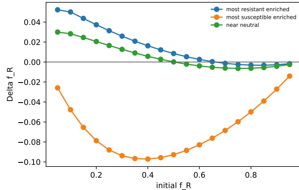
Recovery timing
