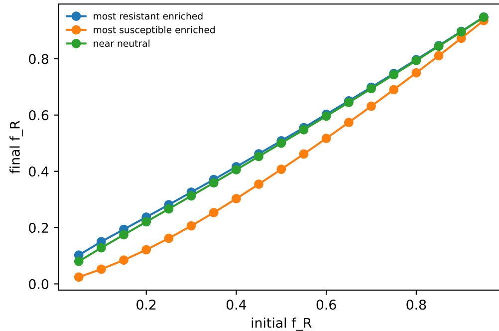
Final diversity
