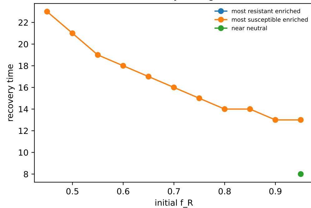
Recovery timing
