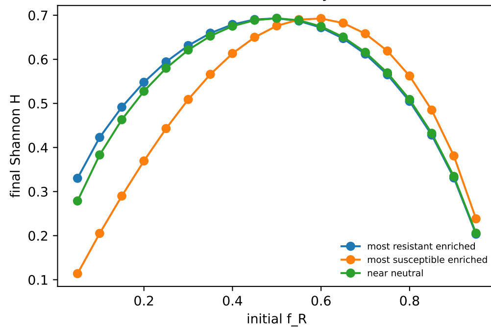
Final diversity
