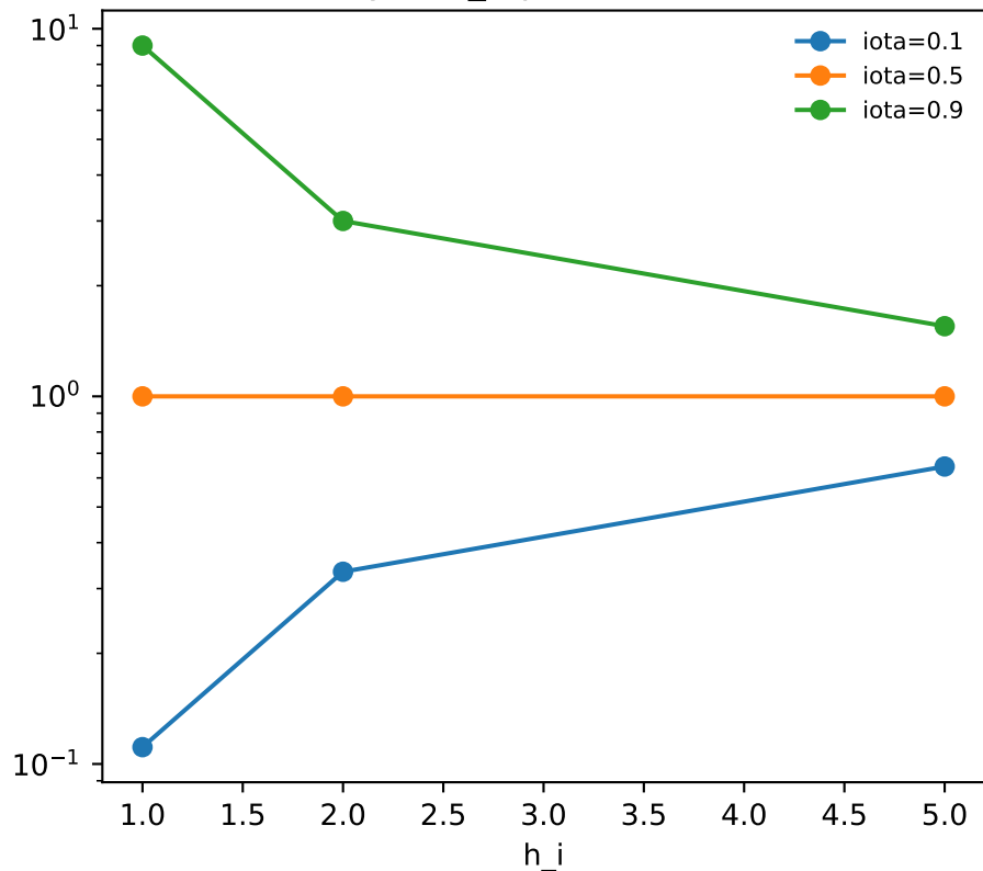
Many (i, h_i) pairs share iota
