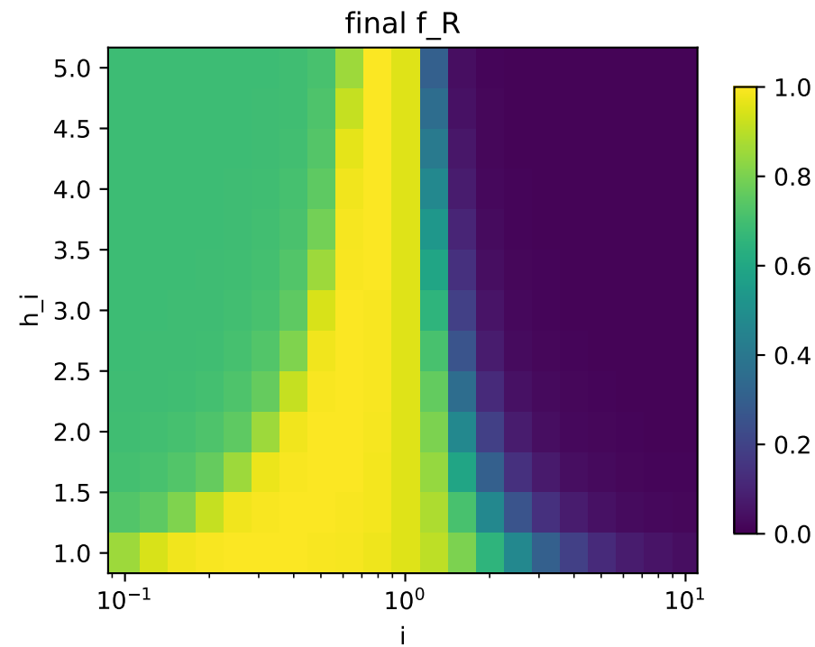
Response atlas: i_{hi} , a_0=100
