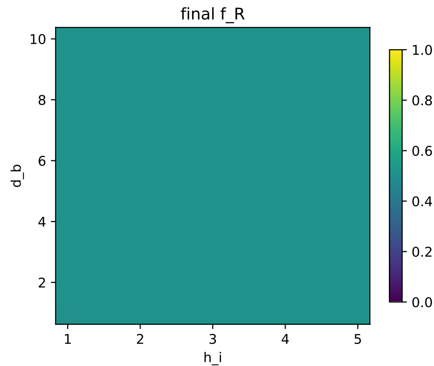
Response atlas: hi_db_i_0.1, a0=2.15
