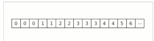
The buffer extraction process for block sort.
