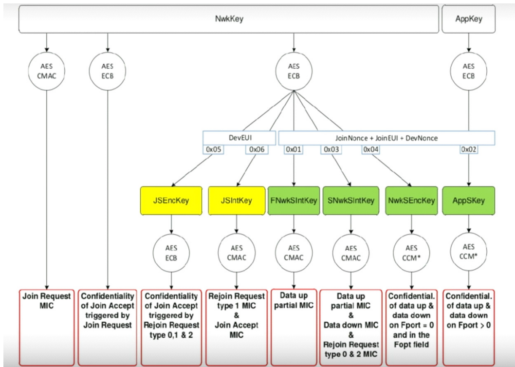
Figure 12-1: Key Derivation Scheme for LoRaWAN 1.1.x
