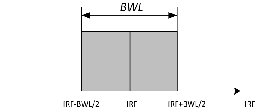
Figure 8-2: LoRa Signal Bandwidth
