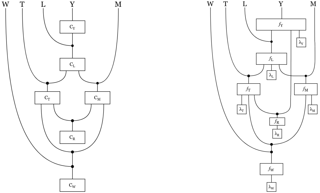
Figure 2: Stage 1 (cont.) — compiled string diagram. The commute model as a Catlab wiring diagram: each variable becomes a mechanism box, copy dots duplicate values feeding several mechanisms, and the shared latent root realises the confounding T \leftrightarrow Y .
