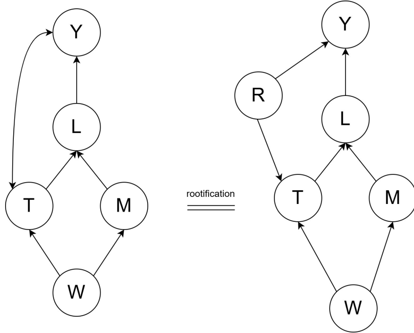
Figure 1: Stage 1 — ADMG compilation (rootification) . The input Acyclic Directed Mixed Graph for the commute model (left) and its rootified form (right), in which the bidirected edge T \leftrightarrow Y is replaced by a fresh latent root R feeding both T and Y .
