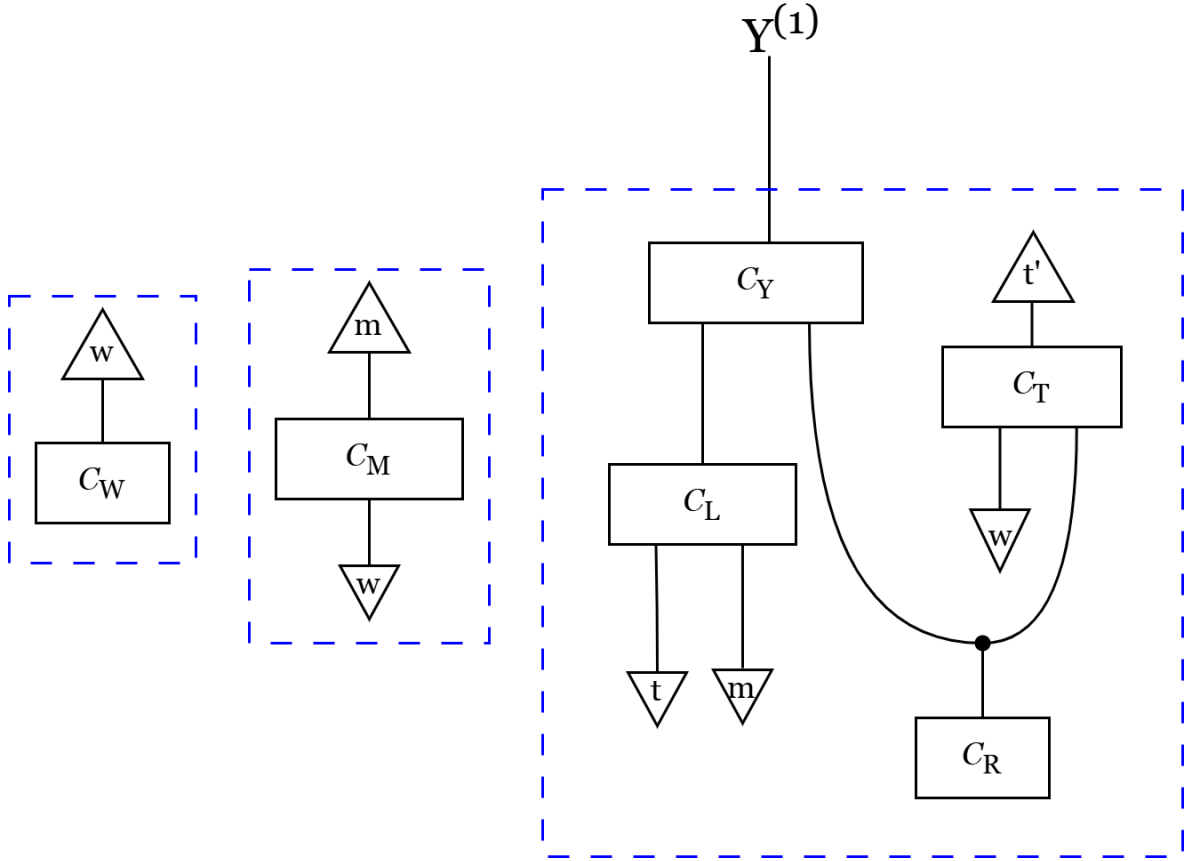
Figure 4: Stage 3 — simplified diagram. The diagram after the four rewrite passes (pruning, observation separation, deterministic-mechanism merging, exogenous-source absorption) reduce it to canonical form.
