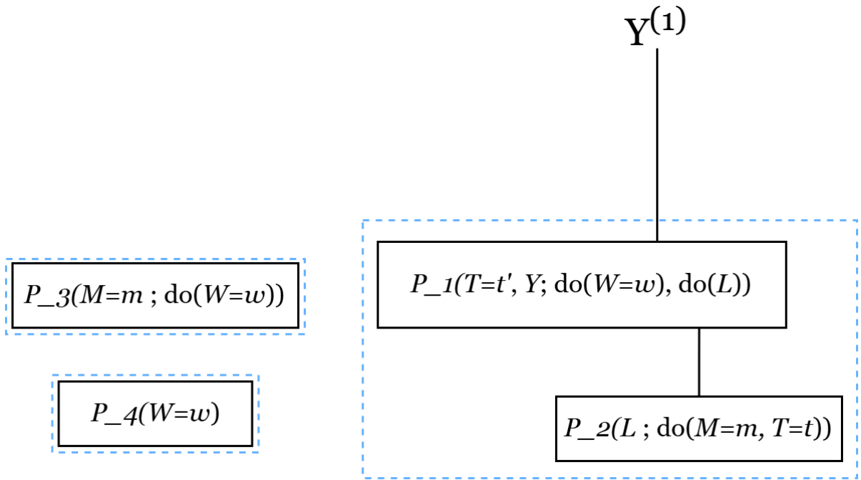
Figure 5: Stages 4–5 — identified estimand. The R-fragments rewritten into interventional probability boxes and rendered as the final estimand. A residual unabsorbed exogenous source would instead signal a non-identifiable query.
