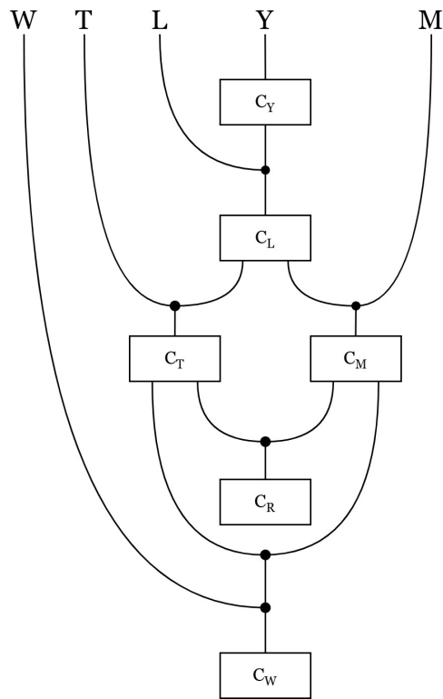
Figure 2: Stage 1 (cont.) — compiled string diagram. The commute model as a Catlab wiring diagram: each variable becomes a mechanism box, copy dots duplicate values feeding several mechanisms, and the shared latent root realises the confounding T \leftrightarrow Y .
