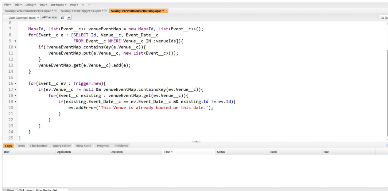
Figure 15. PreventDoubleBooking trigger (double-booking check).
