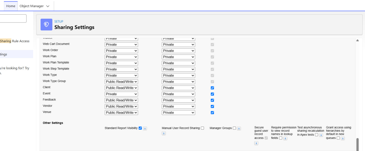
Figure 31. Organization-Wide Defaults for the custom objects.
