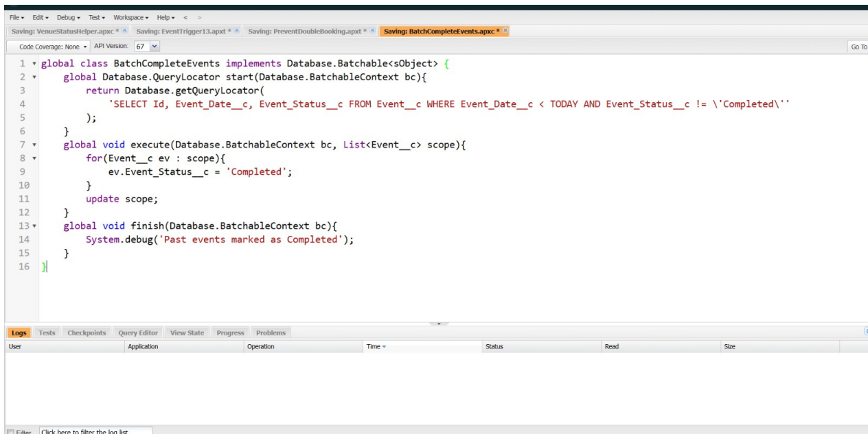
Figure 16. BatchCompleteEvents (Batch Apex).
