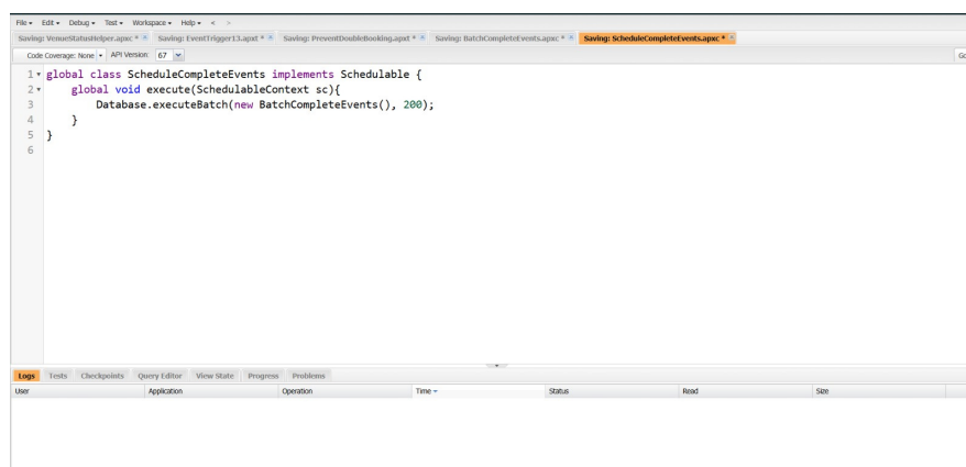
Figure 17. ScheduleCompleteEvents (Schedulable Apex).
