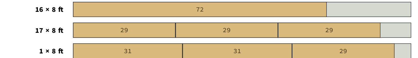
Bars to scale · shaded end is offcut: 24 in, 8¾ in, 4¾ in · kerf not drawn
