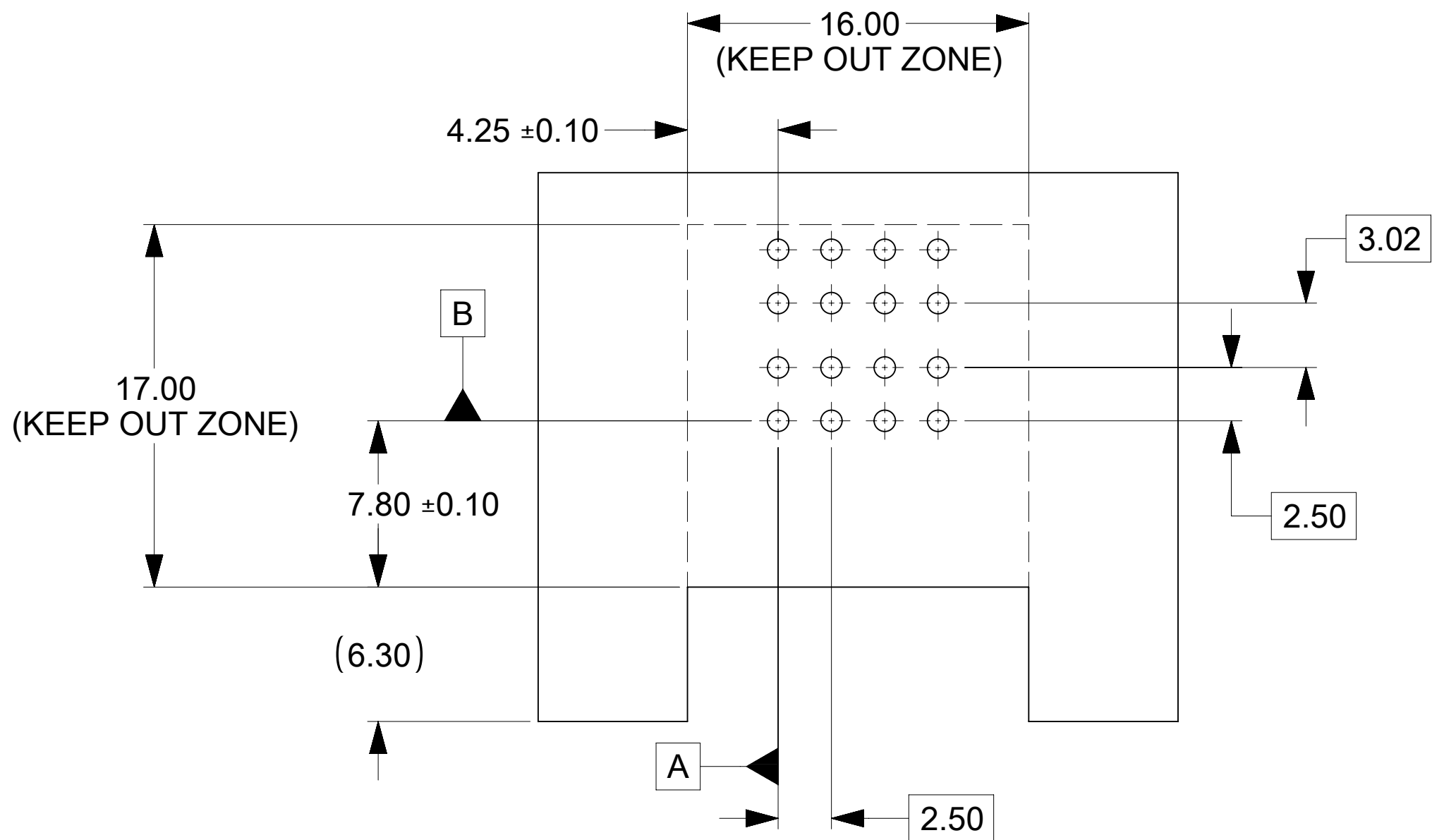
RECOMMENDED PCB LAYOUT AND KEEP OUT ZONE
