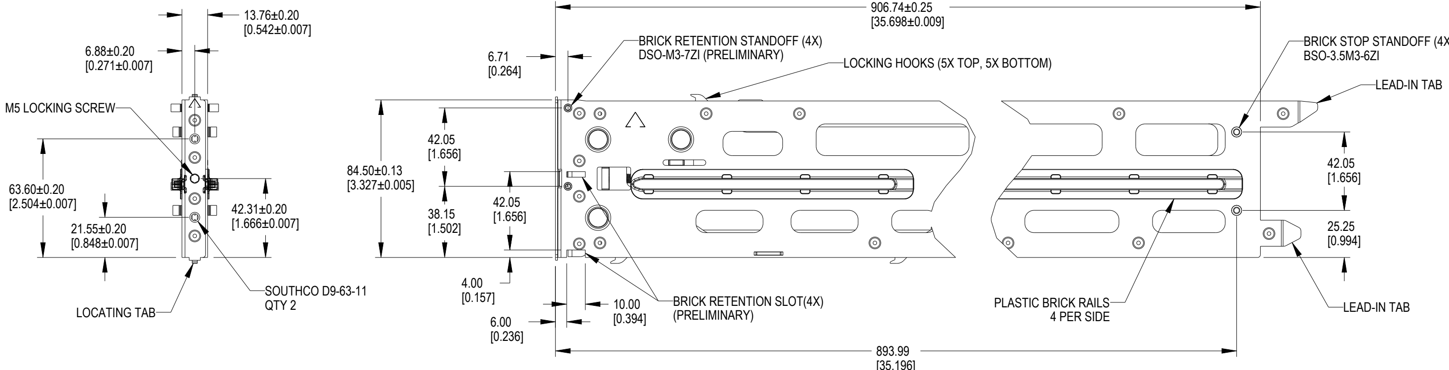
CENTER DIVIDER DETAILS SCALE 0.500
