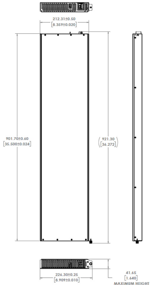
Figure 2 : Brick Dimensions
