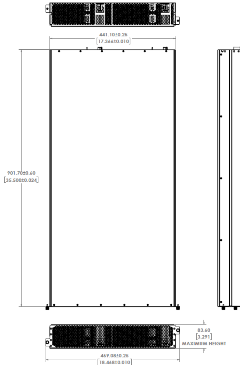
Figure 40 : Double High Double Wide Brick Dimensions
