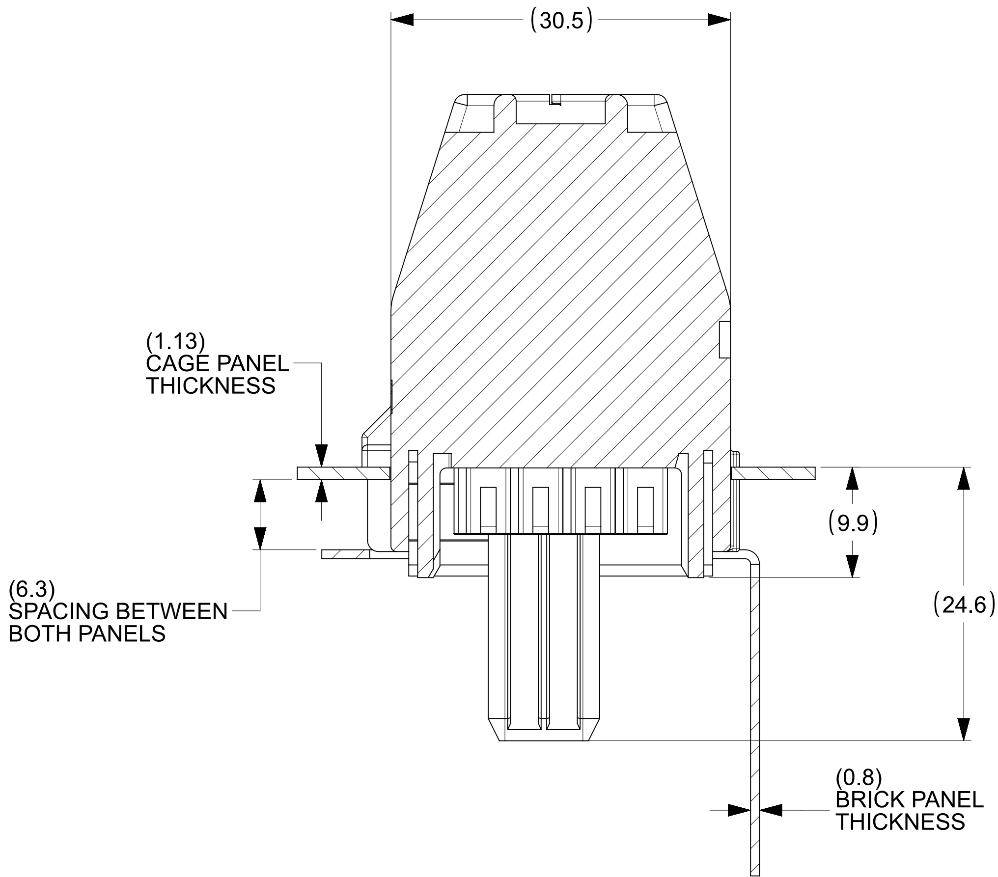
SECTION C-C DATA CABLE IS INTENTIONALLY HIDDEN
