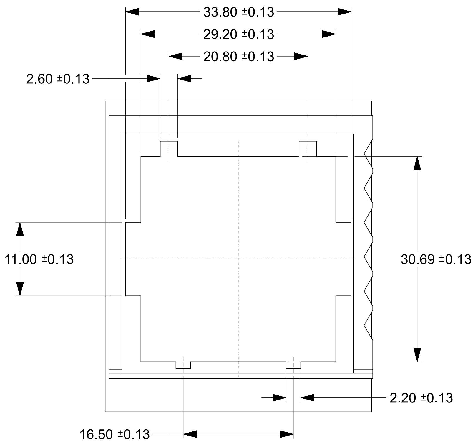
IDEAL PANEL CUT OUT FOR BACKSHELL ASSEMBLY
