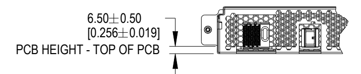
PCB HEIGHT DETAIL REAR VIEW OF BRICK SCALE:0.8
