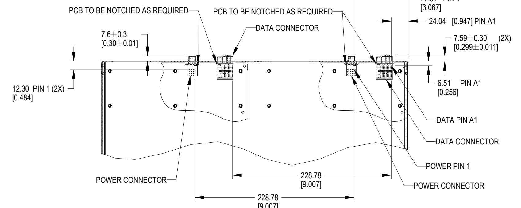
TOP SECTION DATA AND POWER CONNECTION DETAILS
