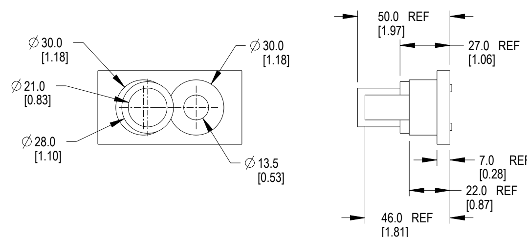
COOLING KEEPOUT ZONE DETAILS SCALE 0.500
