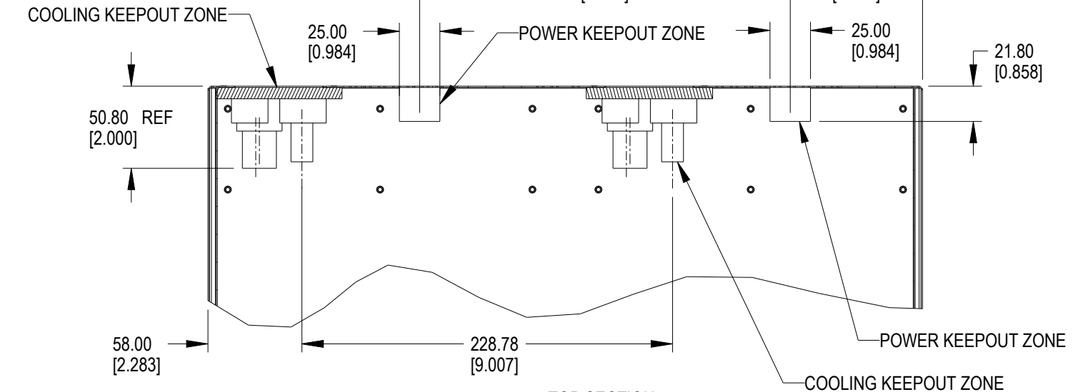
TOP SECTION KEEPOUT ZONE DETAILS
