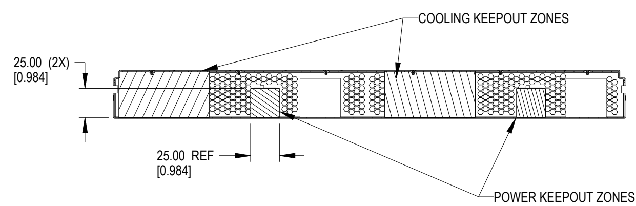
REAR SECTION KEEPOUT ZONE DETAILS
