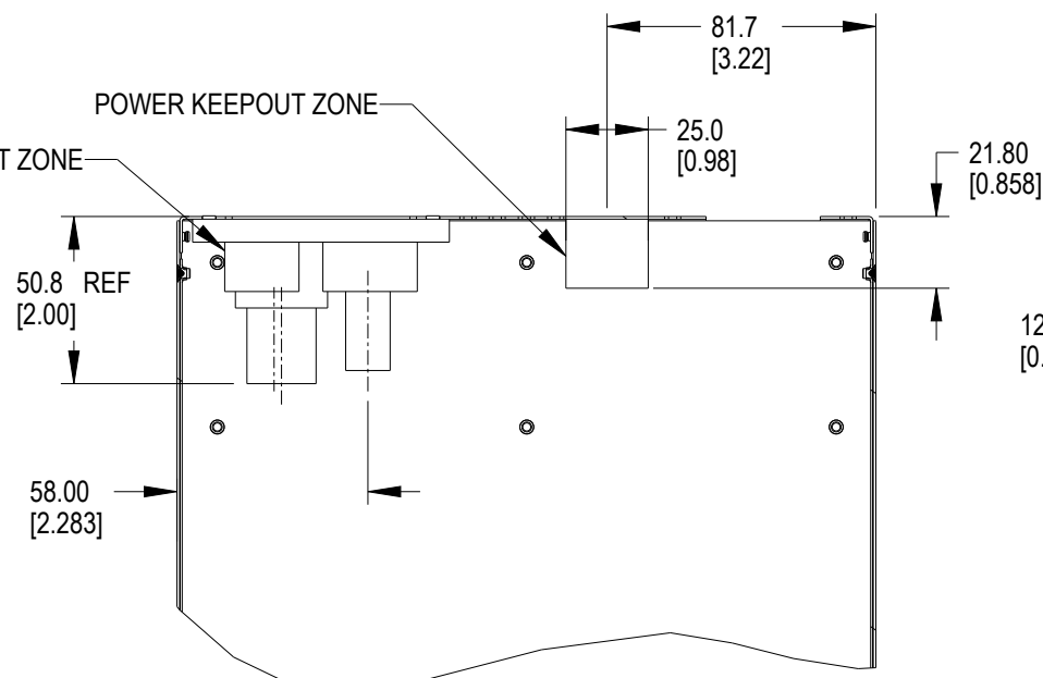
TOP SECTION KEEPOUT ZONE DETAILS
