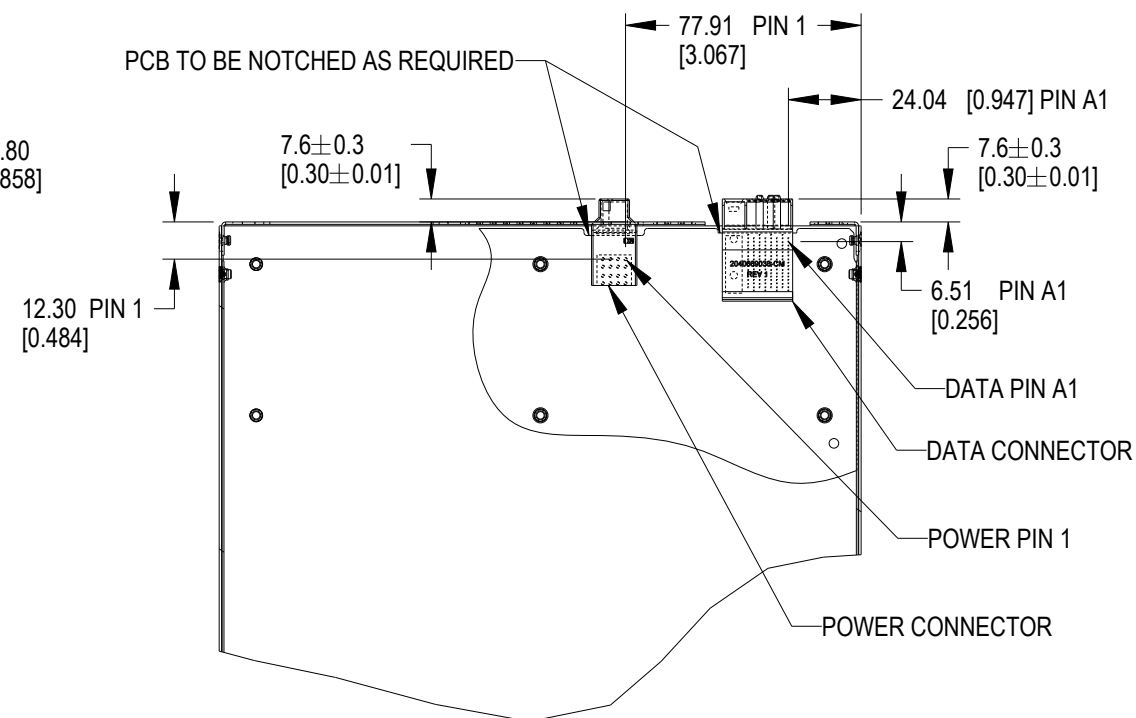
TOP SECTION DATA AND POWER CONNECTION DETAILS
