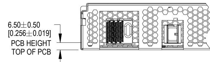
PCB HEIGHT DETAIL REAR VIEW OF BRICK SCALE 1:2
