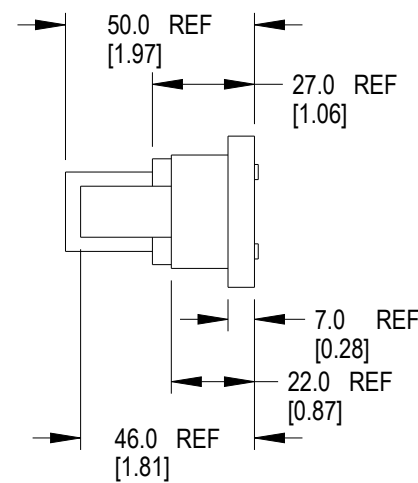
COOLING KEEPOUT ZONE DETAILS SCALE 1:2
