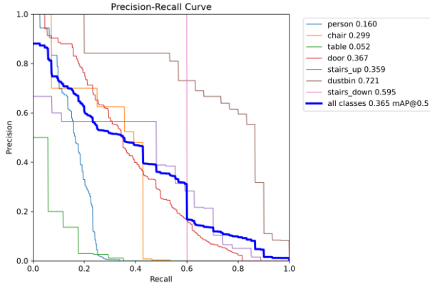
Fig. 4. Precision-recall curves of the AV-7 detector.
