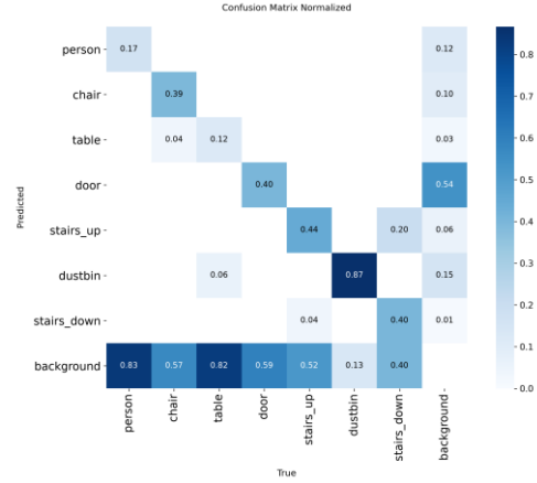
Fig. 5. Normalized confusion matrix of the AV-7 detector.
