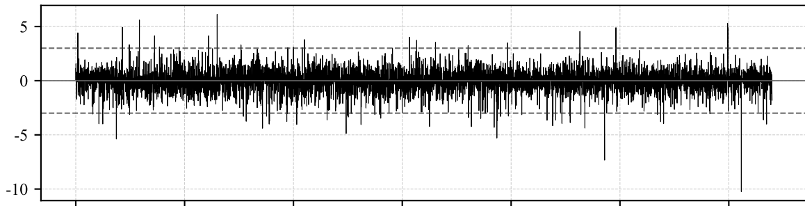
APARCH(1,1)-t 残差 ( \bar{\varepsilon}=-0.006, \hat{\sigma}=1.010 )
