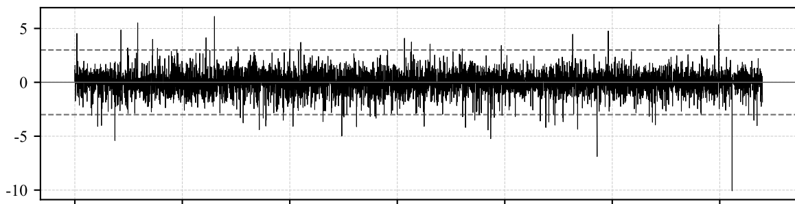
GARCH(1,1)-t 残差 ( \bar{\varepsilon}=-0.006, \hat{\sigma}=0.992 )
