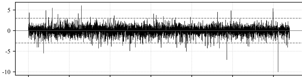
EGARCH(1,1)-t 残差 ( \bar{\varepsilon}=-0.006, \hat{\sigma}=0.995 )
