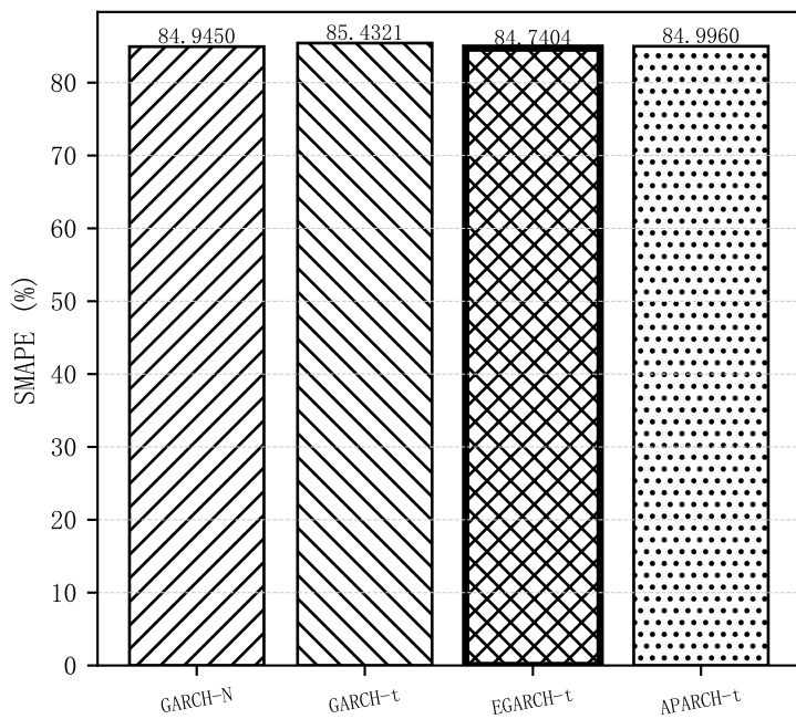
SMAPE (%)
