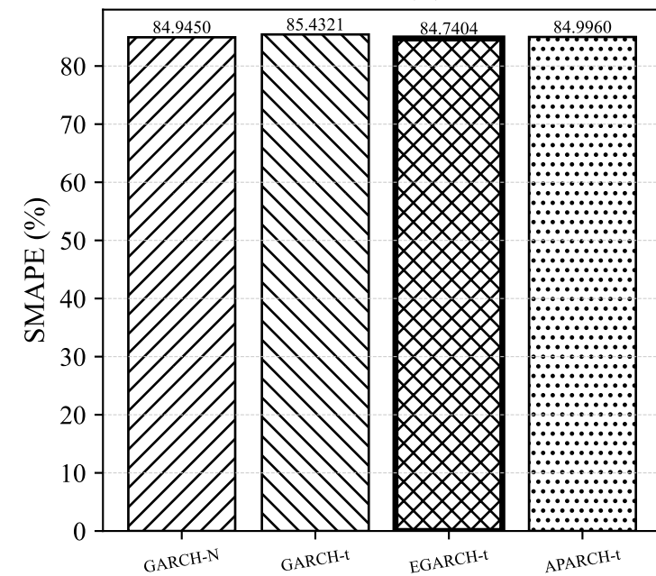
SMAPE (%)
