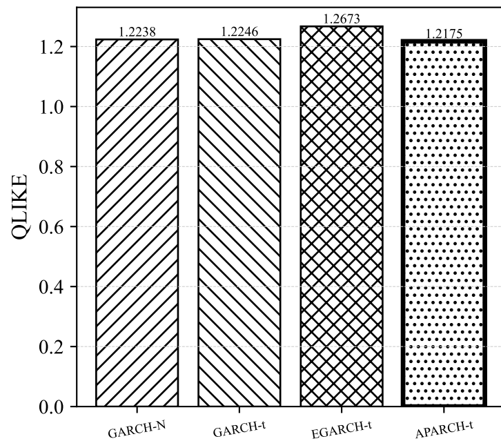
QLIKE
