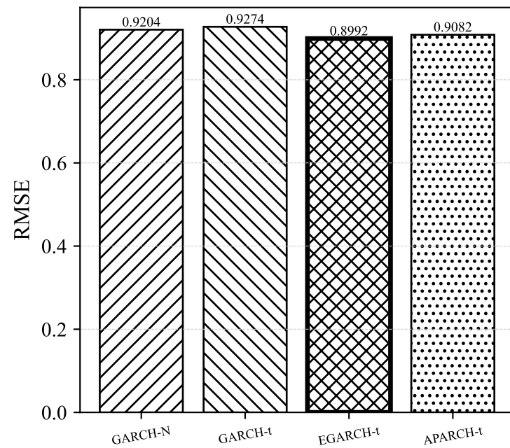
RMSE
