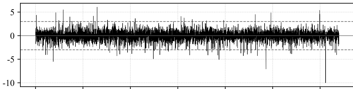
GARCH(1,1)-t 残差 ( \bar{\mu}=-0.006, \hat{\sigma}=0.992 )
