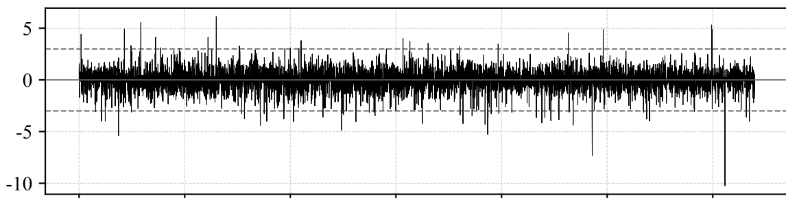
APARCH(1,1)-t 残差 ( \bar{\mu}=-0.006, \hat{\sigma}=1.010 )
