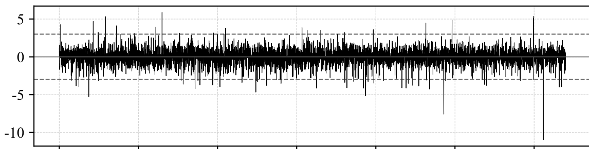
EGARCH(1,1)-t 残差 ( \bar{\mu}=-0.006, \hat{\sigma}=0.995 )
