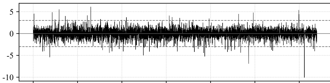
GARCH(1,1)-N 残差 ( \bar{\mu}=-0.007, \hat{\sigma}=1.000 )
