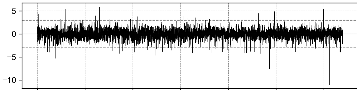
EGARCH(1,1)-t 标准化残差 ( \mu \square = -0.006 , \sigma \square = 0.995 )
