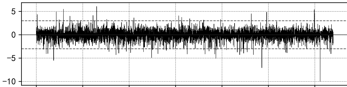
GARCH(1,1)-t 标准化残差 ( \mu \square = -0.006 , \sigma \square = 0.992 )
