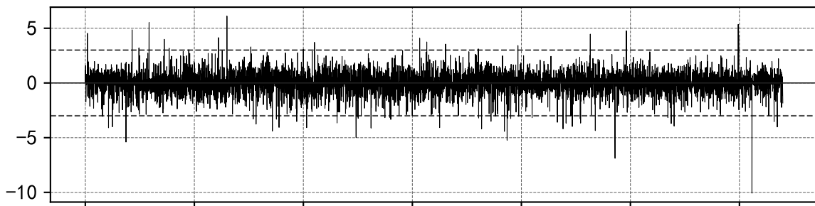
GARCH(1,1)-N 标准化残差 ( \mu \square = -0.007 , \sigma \square = 1.000 )
