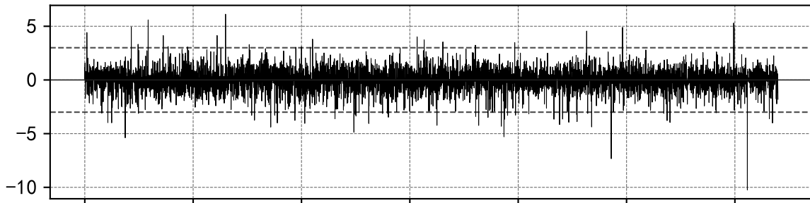
APARCH(1,1)-t 标准化残差 ( \mu \square = -0.006 , \sigma \square = 1.010 )
