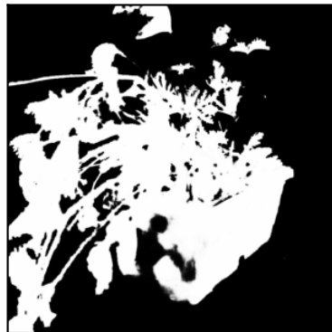
SMat+GF
