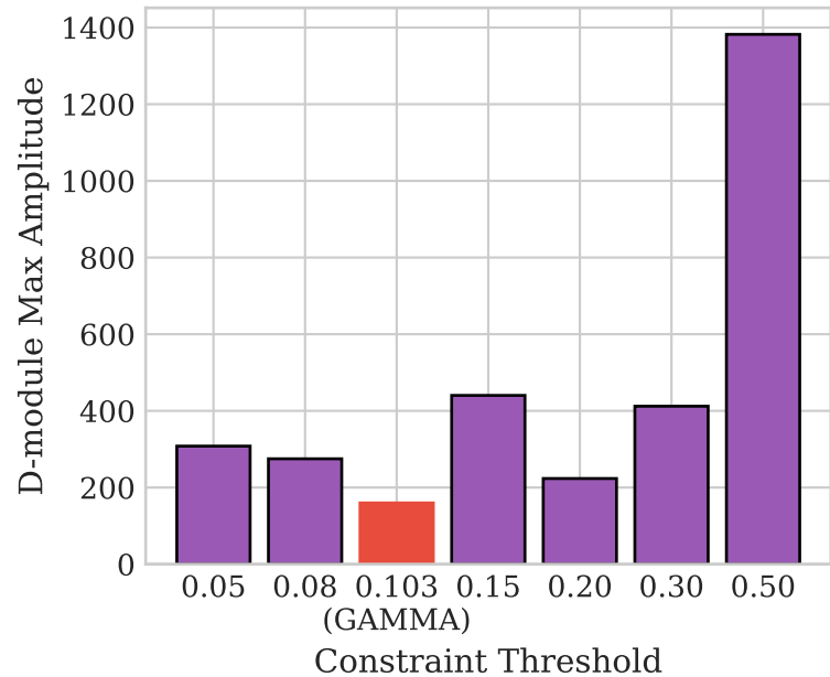
(c) D-module Max (lower is better)
