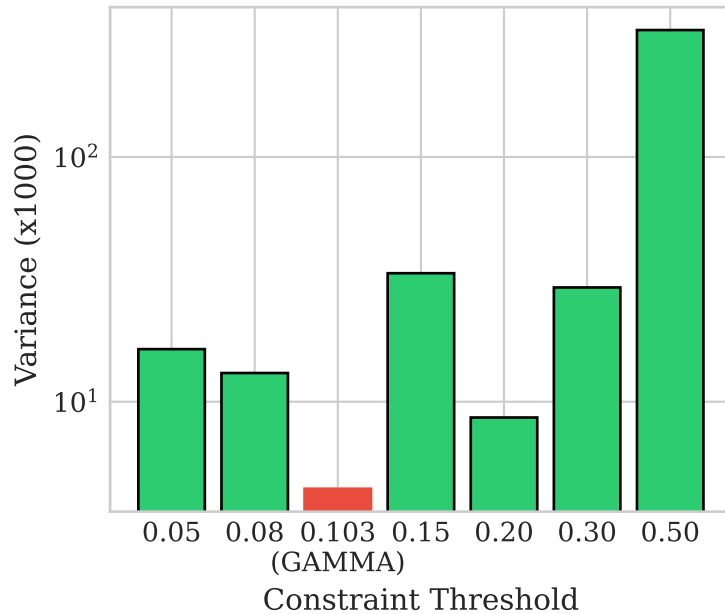
(b) Variance (lower is better)
