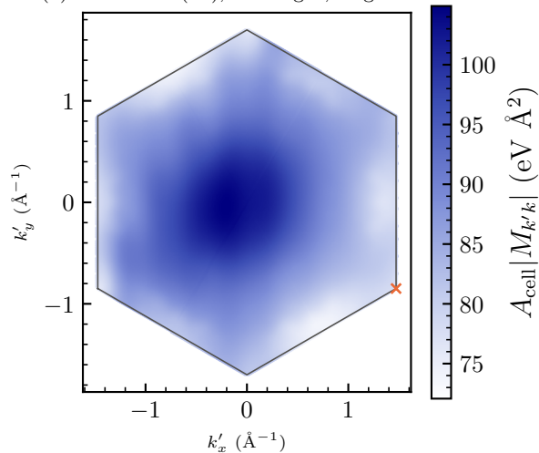
(b) conduction ( \pi^* ), non align , Wigner-Seitz
