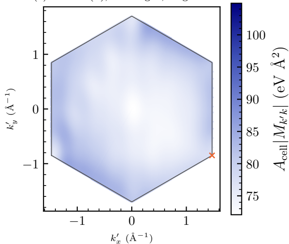
(a) valence ( \pi ), non align , Wigner-Seitz
