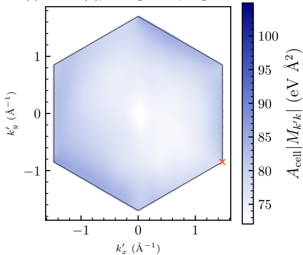
(c) valence ( \pi ), Kumagai-Oba, Wigner-Seitz
