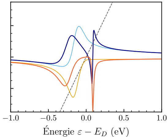
(b) Kumagai–Oba, c_i = 1\% , k = K
