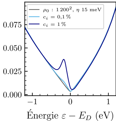
(a) \rho(\varepsilon) , tel quel
