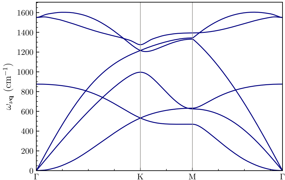
(a) 24 \times 24 \mathbf{k} , 24 \times 24 \mathbf{q} , \sigma_{MV} = 0.02 \text{ Ry}
