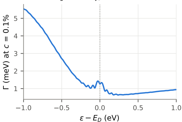
(e) vacancy, c = 0.1\% (vs Kaasbjerg Fig. 17: subst. N, order of magnitude only)
