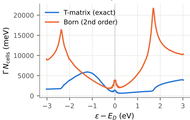
9x9: on-shell rate, \eta = 0.02 eV
