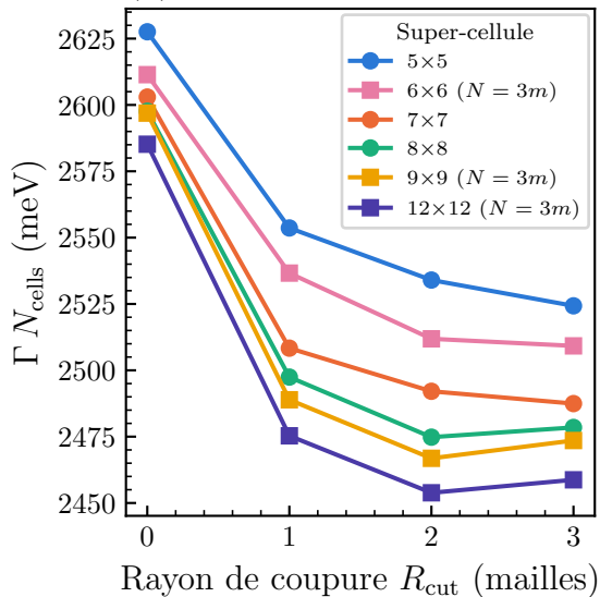
(a) Grille k 240 \times 240 , \eta = 0.02 eV
