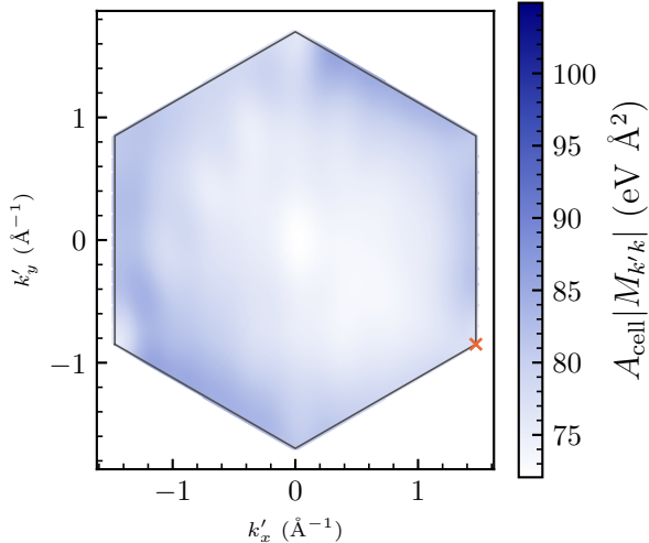
(a) valence ( \pi ), M2 tel quel
