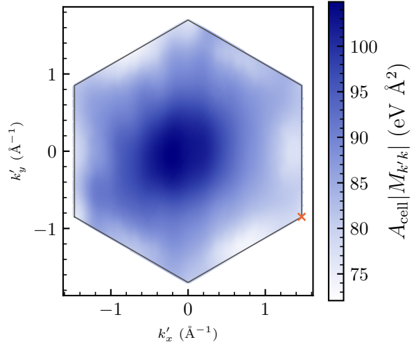
(b) conduction ( \pi^* ), M2 tel quel
