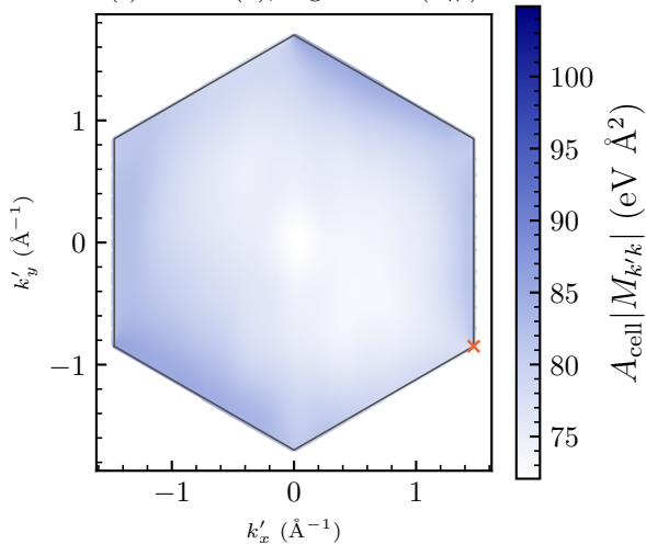
(c) valence ( \pi ), align  exact ( F_W )
