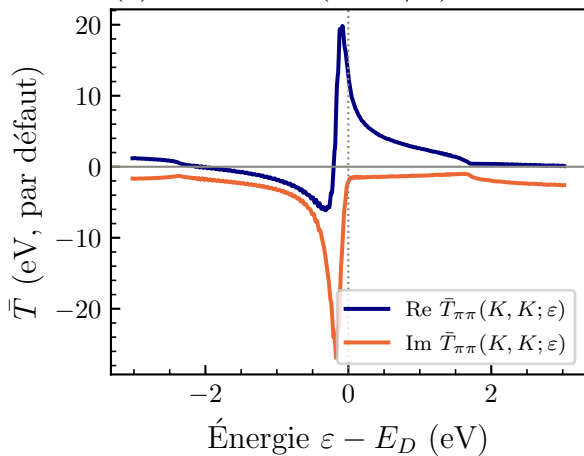
(c) \bar{T}_{\pi\pi} en K (trace/2)
