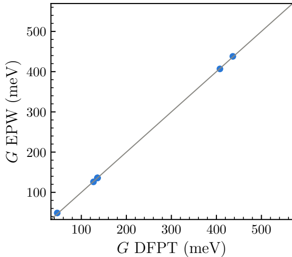
(a) \mathbf{k} = \Gamma
