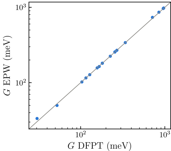
(b) \mathbf{k} = K
