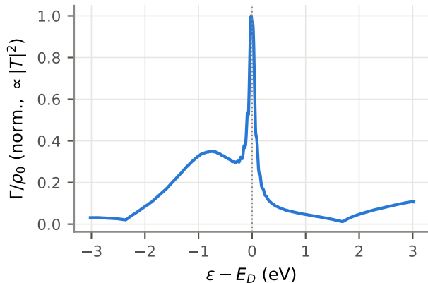
(a) \Gamma(\varepsilon)/\rho_0(\varepsilon)
