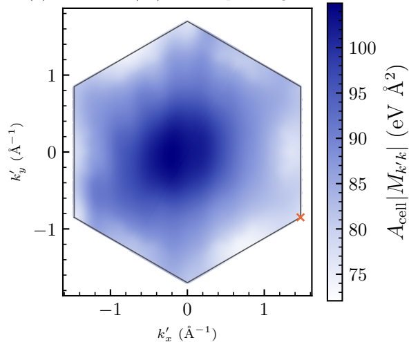
(b) conduction ( \pi^* ), M2 tel quel, Wigner-Seitz
